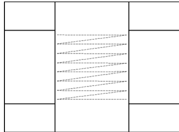
14 point stitching (7 points on each side) reinforces strength of 4" webbing
